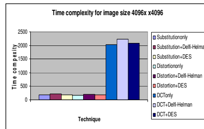
Figure 5(f). Time Complexity (4096X4096 pixel)
