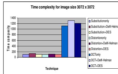
Figure 5(d). Time Complexity (3072X3072 pixel)
