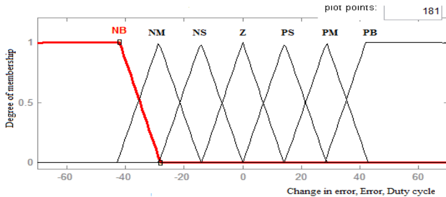
Fig. 7 Membership functions of fuzzy controller.
