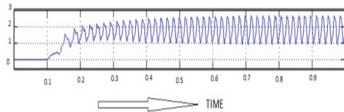
Fig. 11(b) Torque response using Fuzzy with reference set speed 1500rpm.
