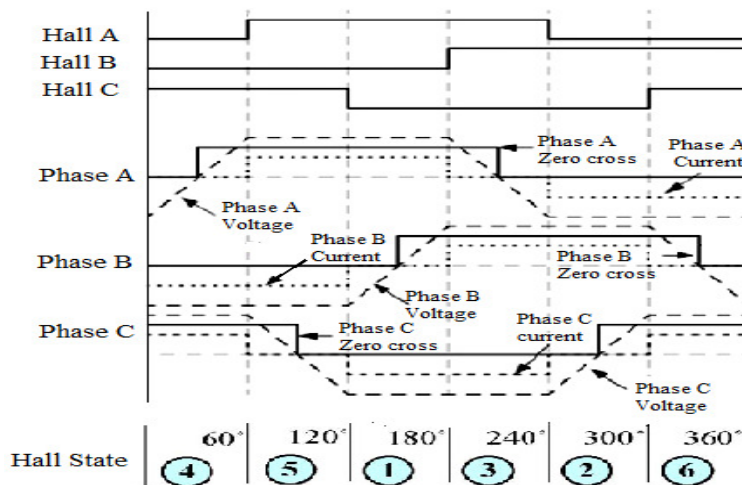
Fig. 3 Waveform of Back EMF and phase current with respect to Hall state.
